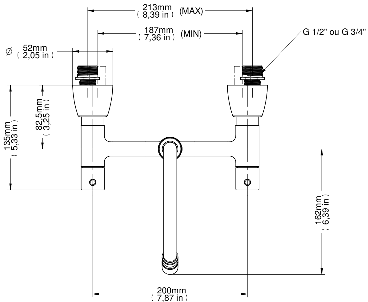
MISTURADOR P/ PIA DE COZINHA PAREDE 1/2" ALAVANCA ALAVANCA WALL MOUNT MIXING SET 1/2" MEZCLADOR DE PARED ALAVANCA 1/2"
